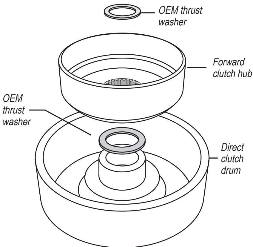
Forward clutch drum side
