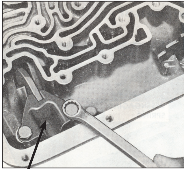
PARK LOCK BRACKET
